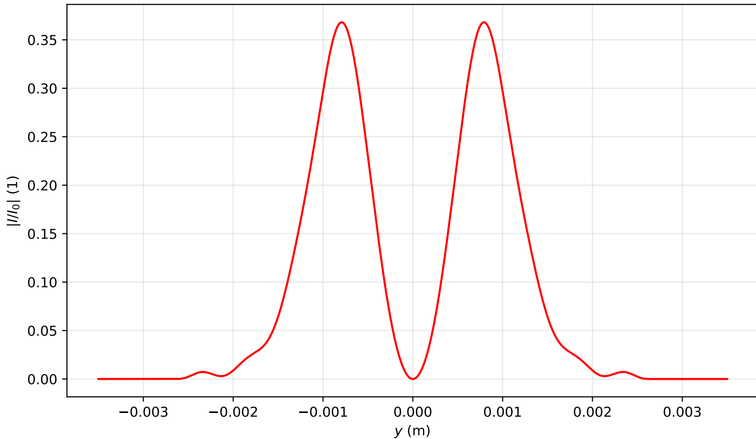
Intensity profile I(x=0, y, z=3.184)/I_0 , \text{Pin}=3.0\text{Pcr} , artificial time
